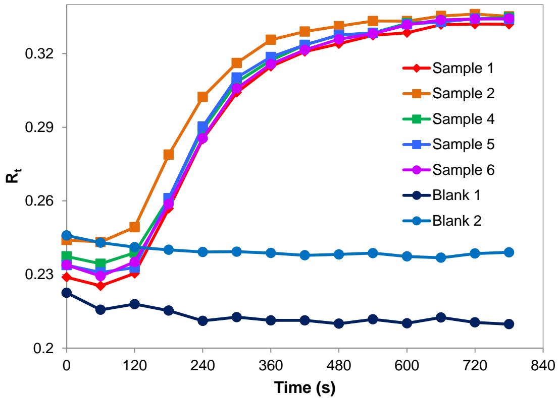
Figure 3. – The normalised red component ( R_t ) vs. time curves for 5 of the best samples (from 8). The average, standard deviation and % standard deviation ( \sigma/\mu \times 100 ) are shown below:
